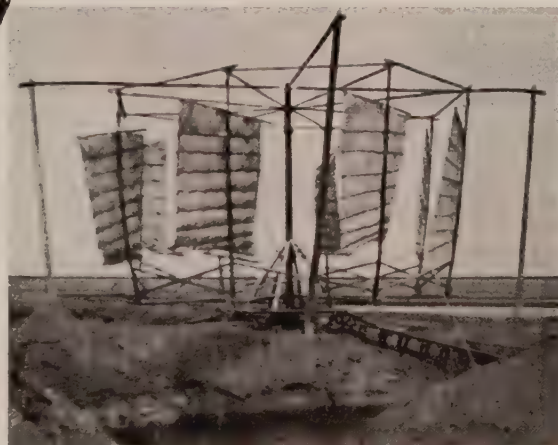
Fig. 689. Typical Chinese horizontal windmill working a square-pallet chain-pump in the saltens at Taku, Hopei (king, 3). The fore-and-aft mat-and-batten type sails luff at a certain point in the cycle and oppose no resistance as they come back into the eye of the wind (see diagram on p. 559)
